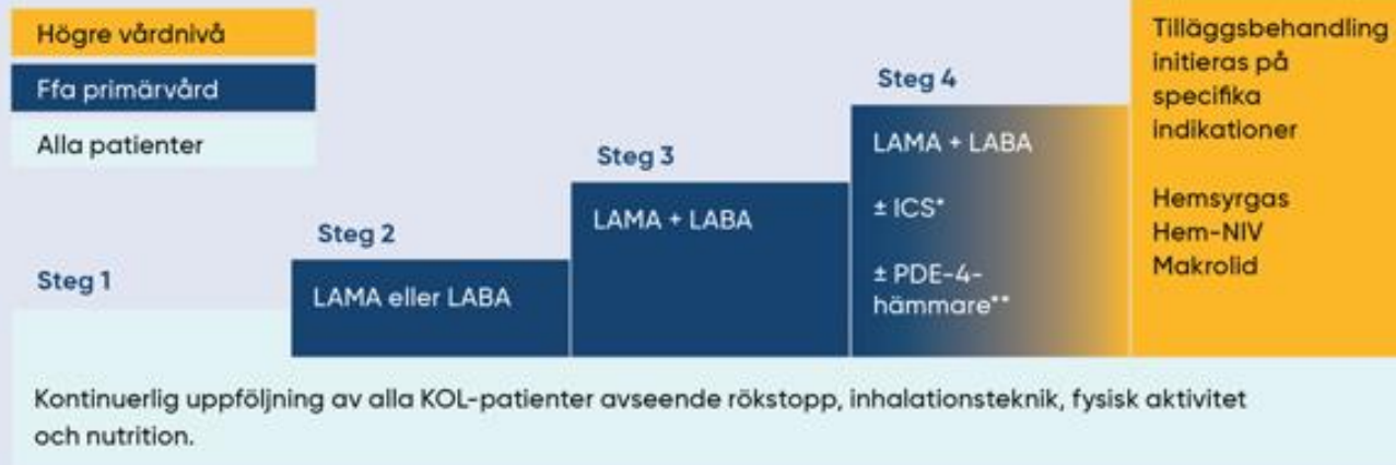
Figur 4. Behandlingstrappan KOL.
